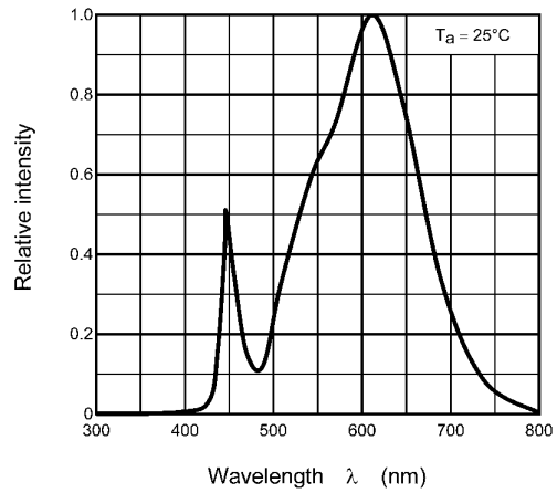
Fig. 8.4 Wavelength characteristic
